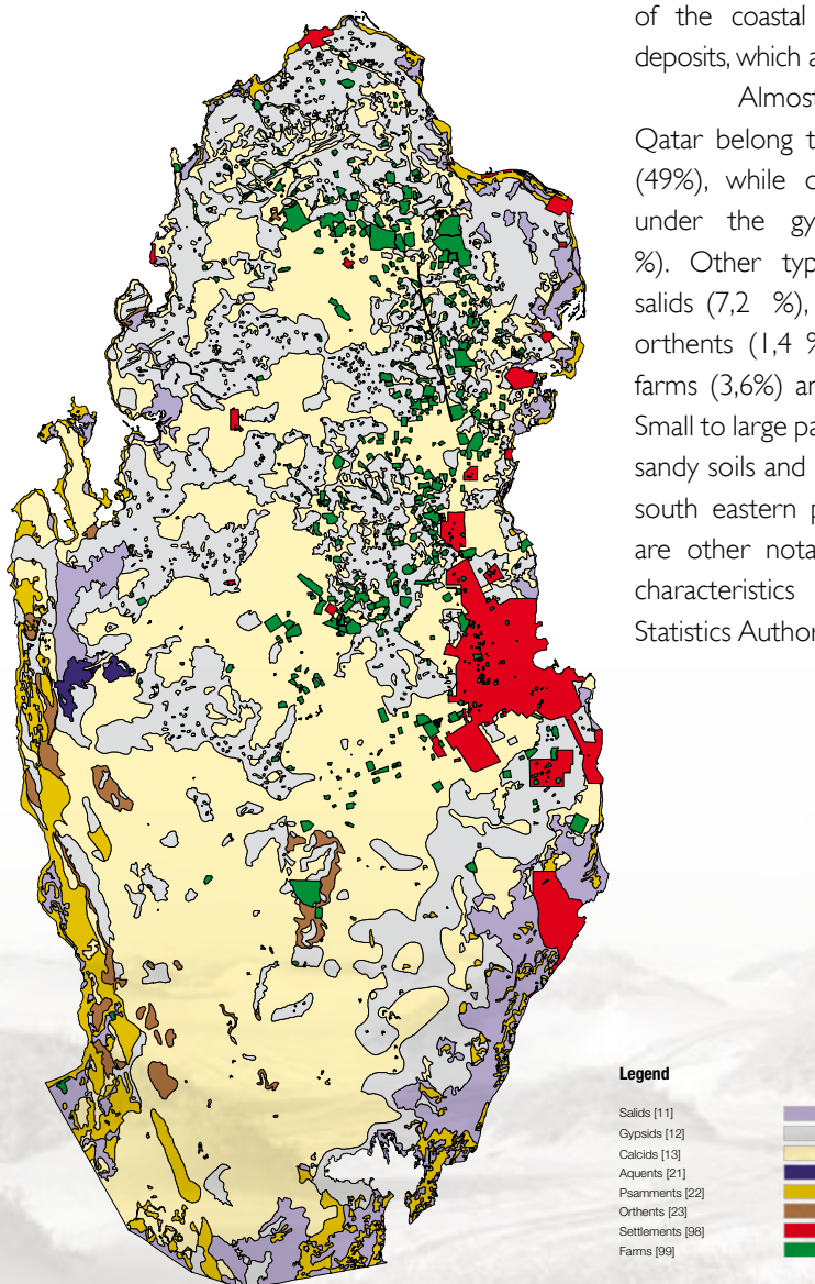
Soil map of Qatar. See legend for interpretation
