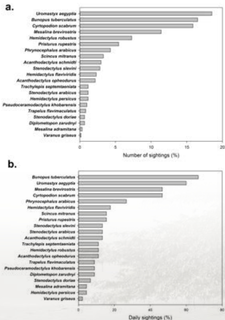
Figure 5. Estimates of lizard species richness based on (a) the proportion of sightings of a certain species from the total number of sightings (n = 617), and (b) the presence of a species per day from the total number of fieldwork days (n = 45)(Cogălniceanu et al. 2014)
