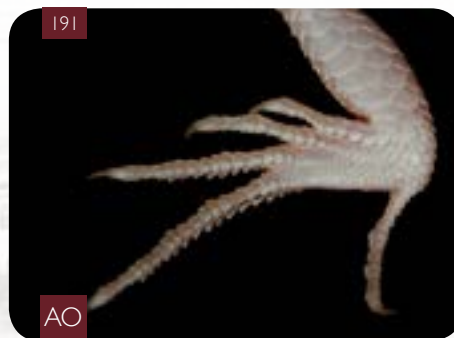
Fringed toes with scales are adapted for running over loose sand. In the photos, Phrynocephalus arabicus (PA), Acanthodactylus schmidtii (AS), Acanthodactylus opheodurus (AO)
